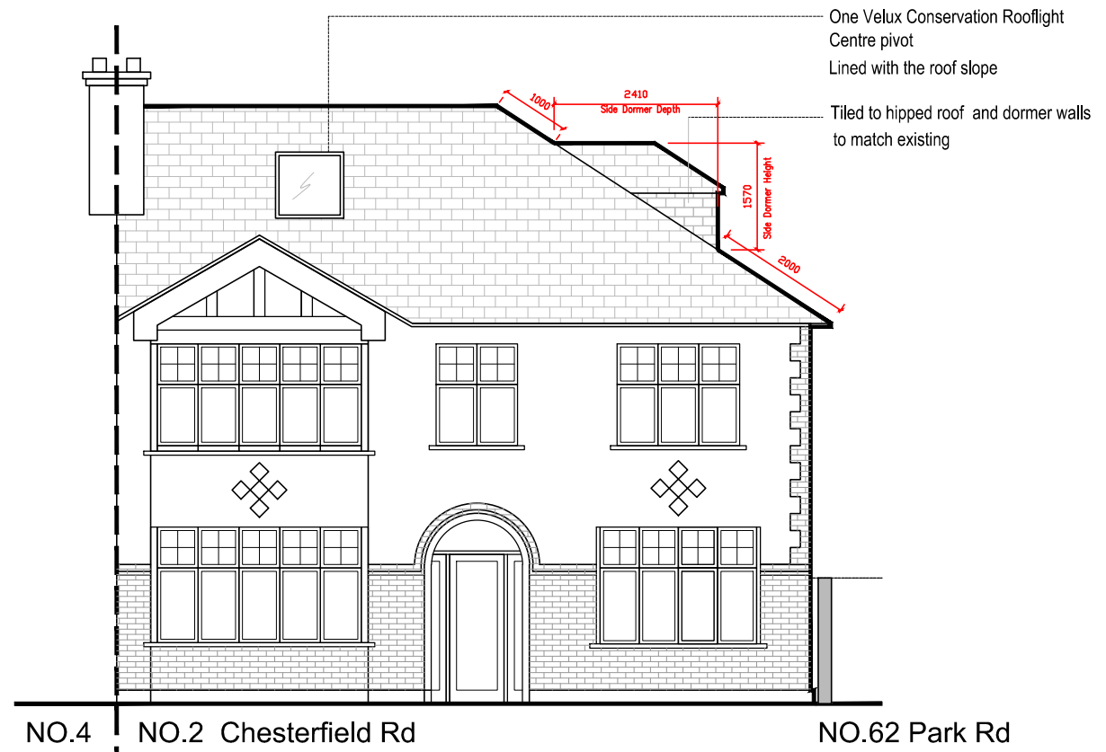
Proposed Front Elevation 1:100@ A3
